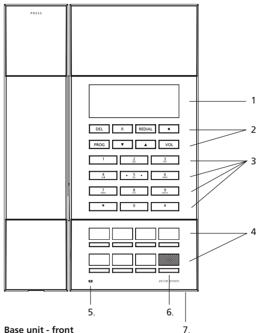
Base unit - front 1. LCD screen display 2. 8 functional keys 3. 12 numerical keys 4. Service buttons 5. Indicator (LED) 6. Message waiting indicator (MWI) 7. Hands-free microphone
